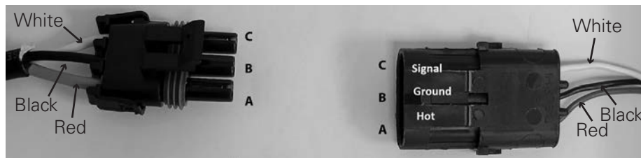
Meter Connection
